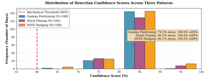
Fig. 8. Distribution of detection confidence scores across three patterns. All patterns show mean confidence above 79% for detected instances, with 100% of detections exceeding the 60% mechanical threshold. Detection counts: gamma positioning (N=168), stock pinning (N=163), ODTE hedging (N=188).
