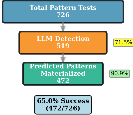
Fig. 9. Pattern detection validation funnel showing progression from 726 total tests to 519 detections (71.5% detection rate) to 472 materialized predictions (90.9% accuracy), yielding 65.0% overall success rate.
